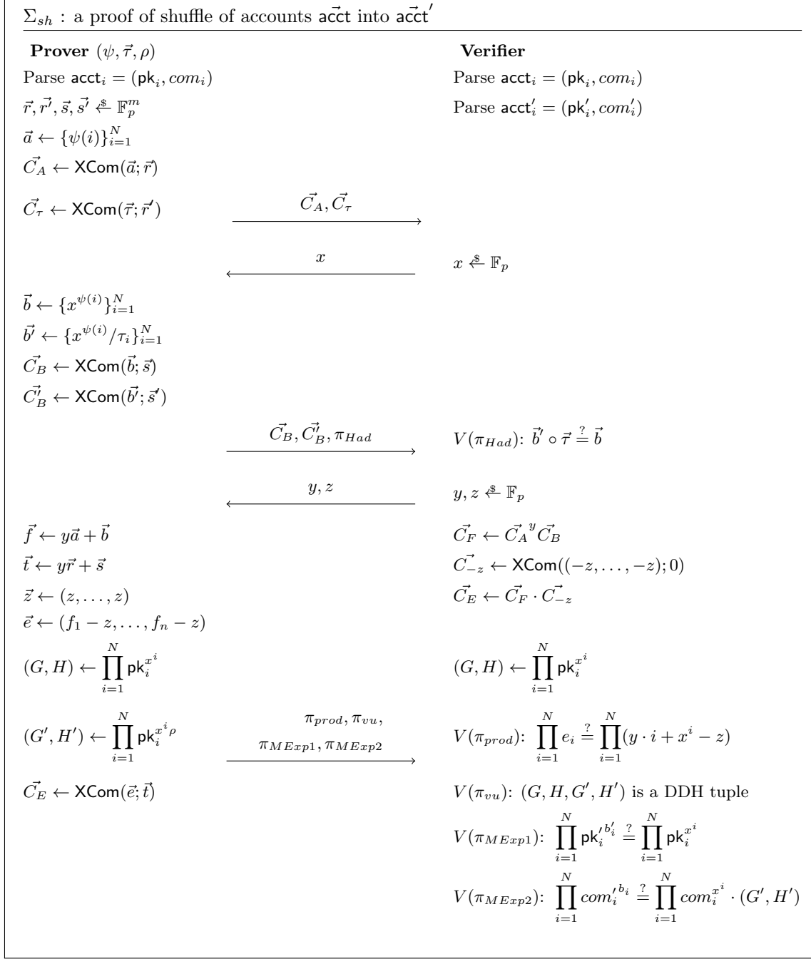
Figure 1: The full shuffle argument \Sigma_{sh} . Here V(\pi) : x means that statement x should be verified using the argument \pi .
