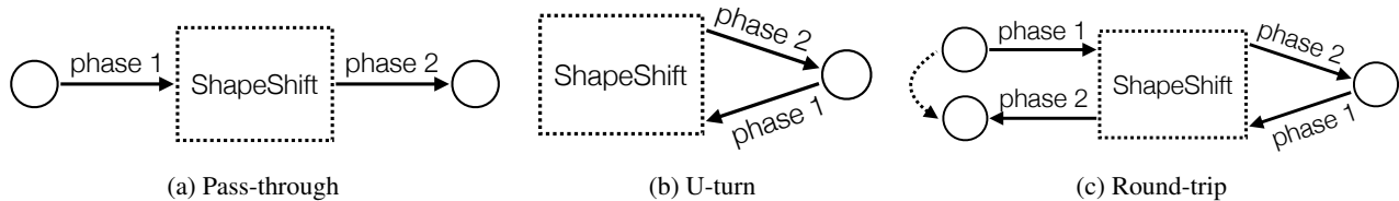
Figure 2: The different transactional patterns, according to how they interact with ShapeShift and which phases are required to identify them.
